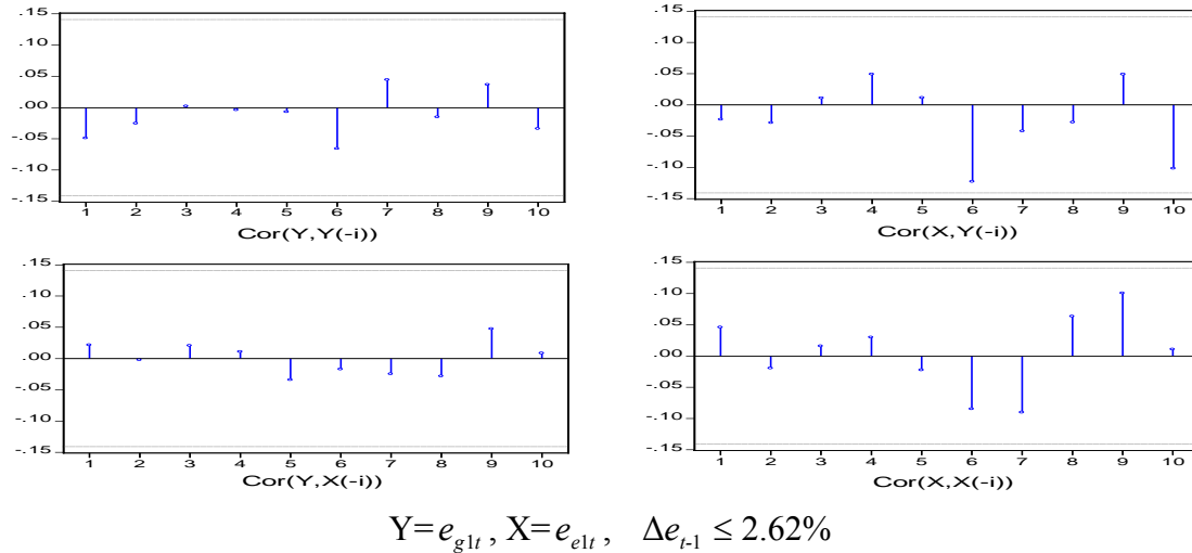
Figure 3. Autocorrelation and cross-correlation analysis using residuals of the TVAR model
